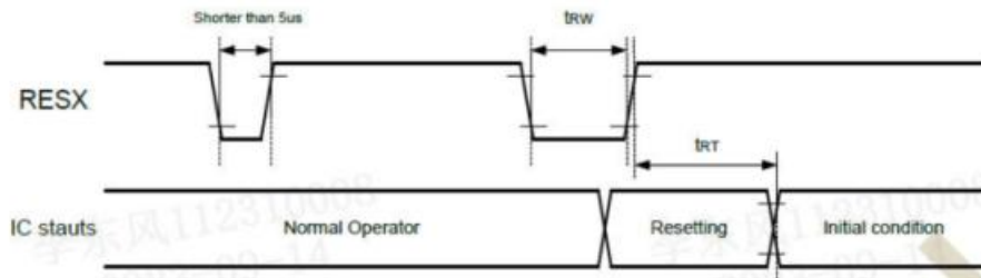
Figure 12.1: Reset input timings
