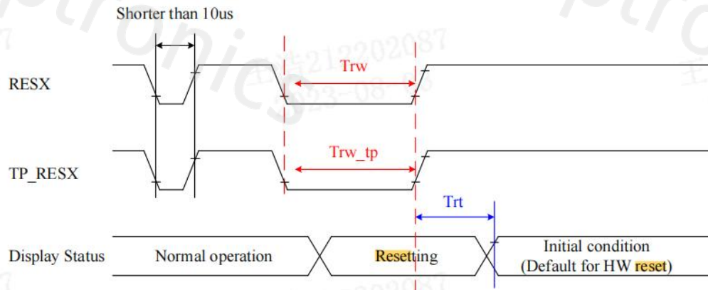
Figure 90. Reset Timing
